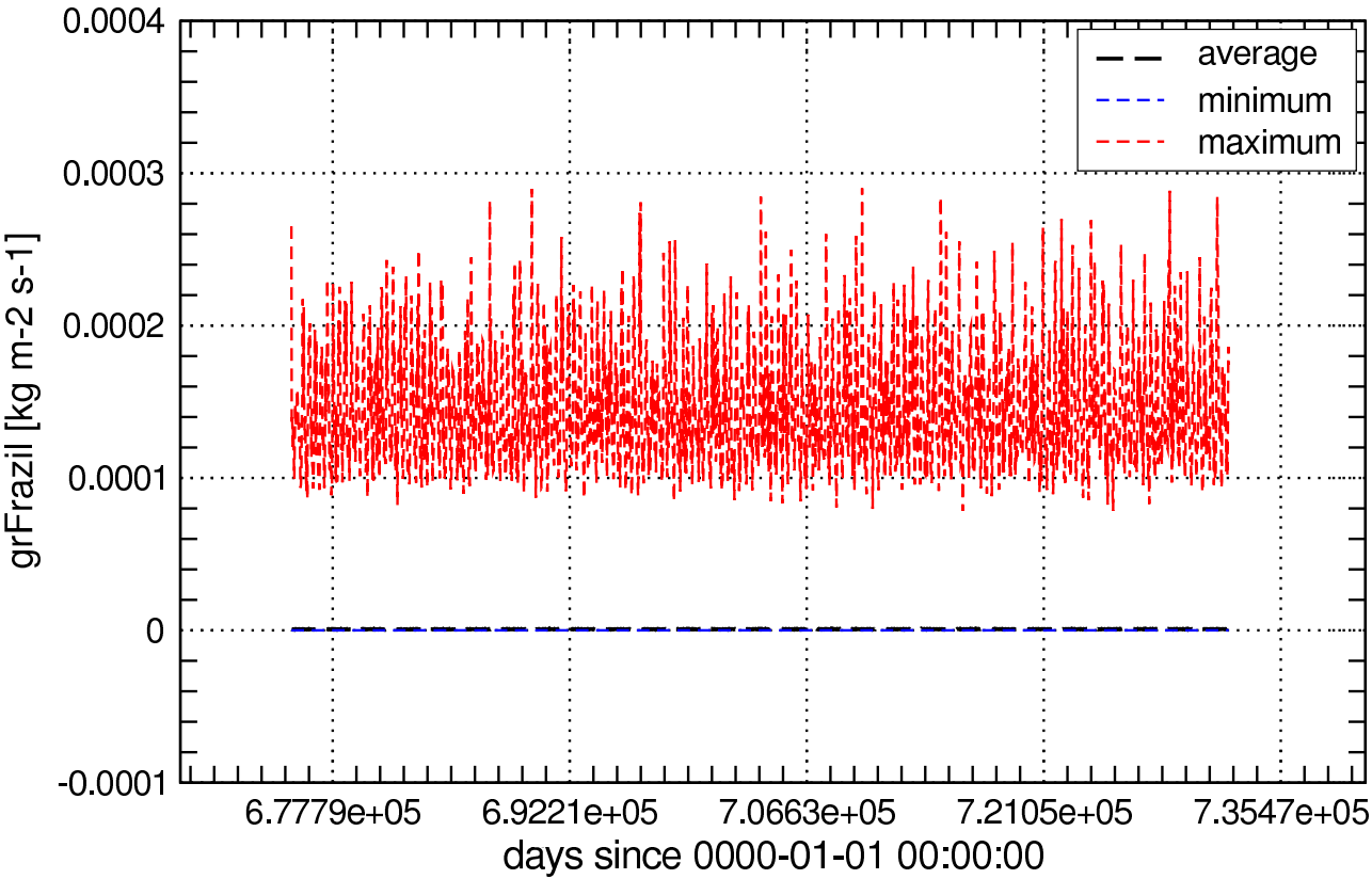
Global Values of grFrazil_Olmon
