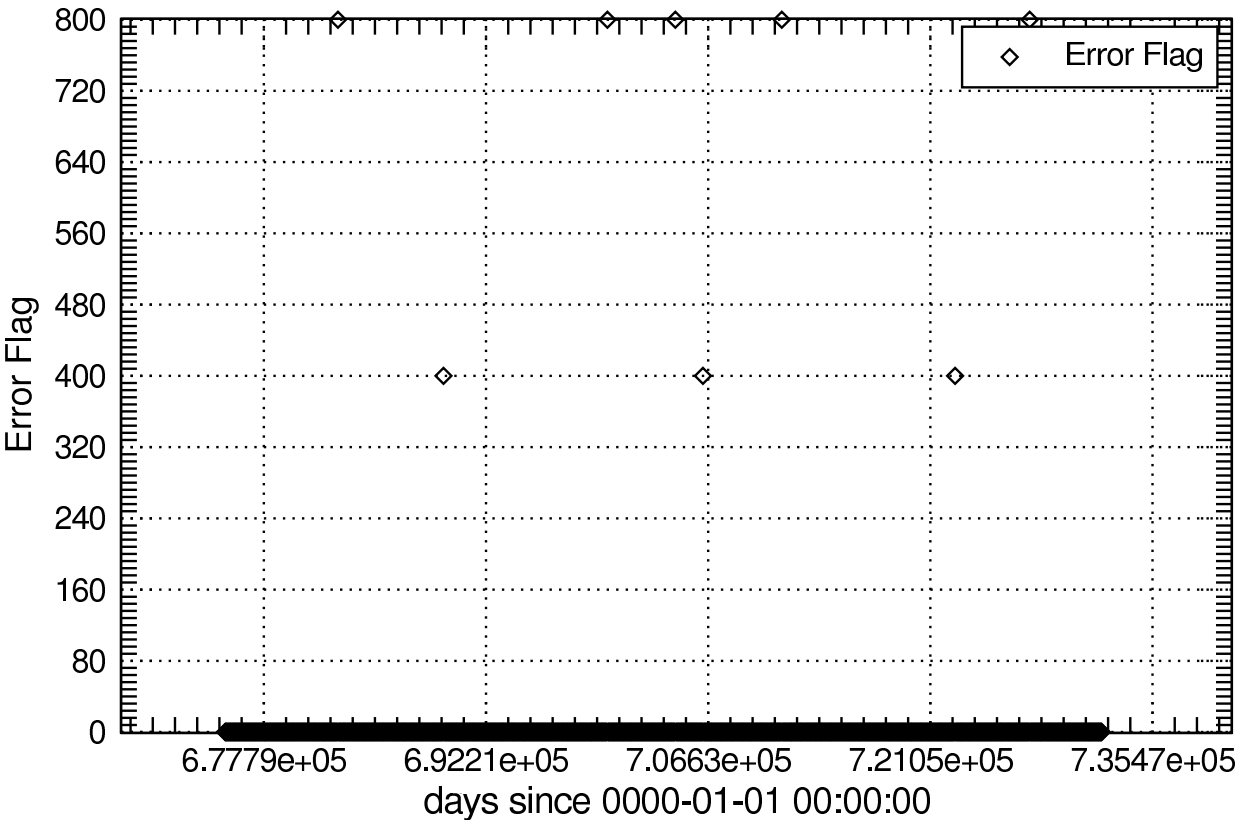
Error Flag of divice_Olmon
