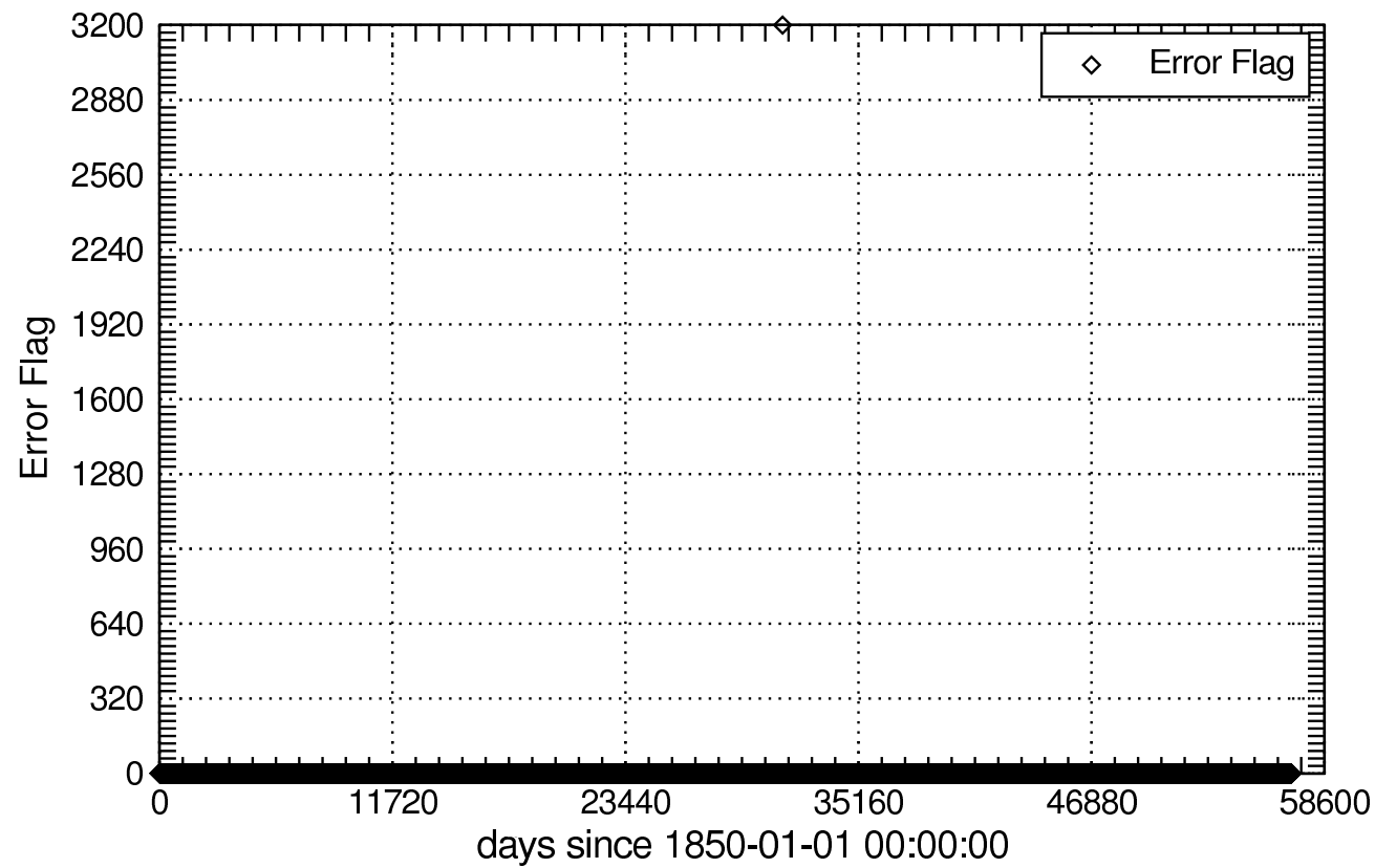
Error Flag of tasmax_day
