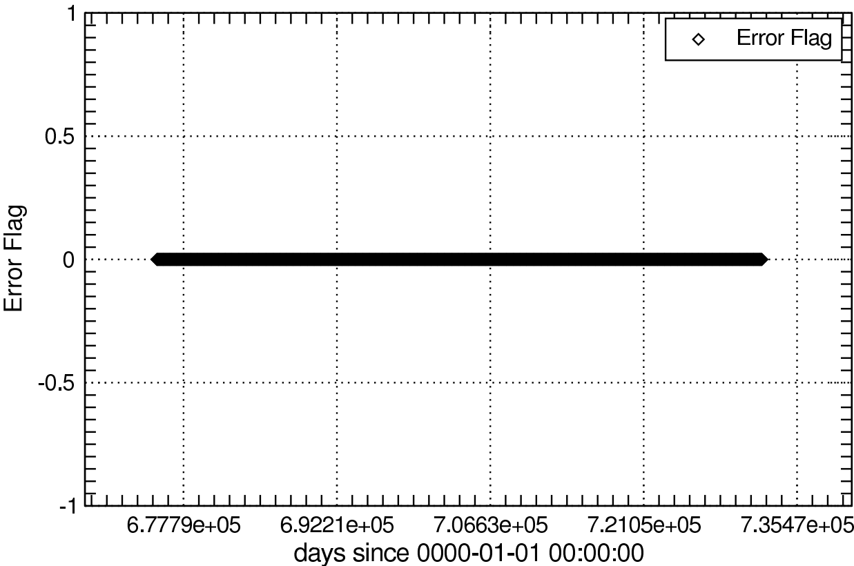
Error Flag of grCongel_Olmon
