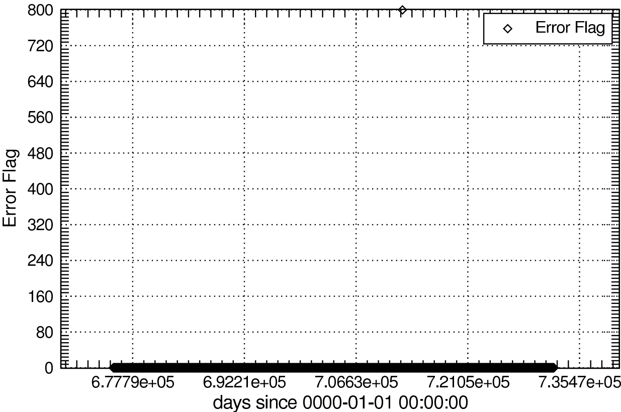
Error Flag of grFrazil_Olmon
