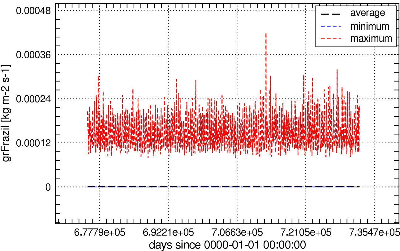
Global Values of grFrazil_Olmon
