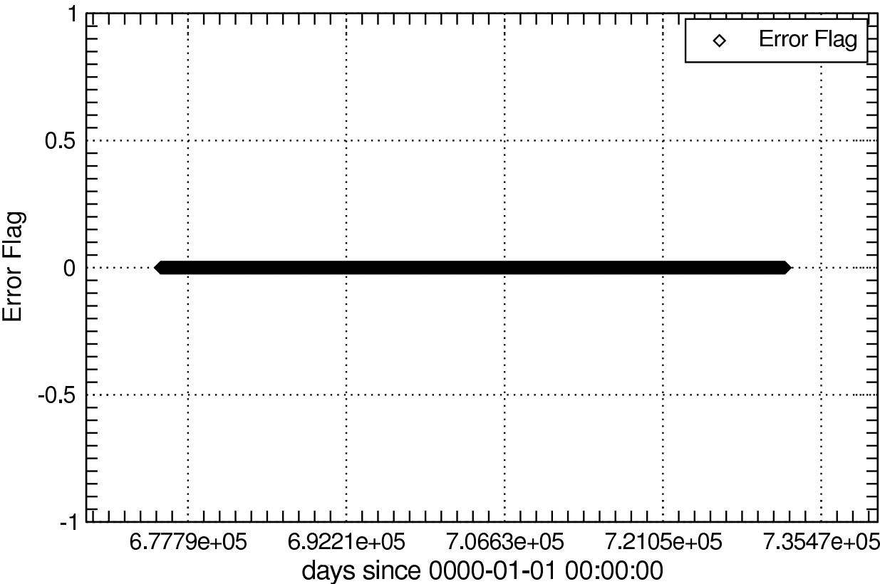
Error Flag of sog a _Omon
